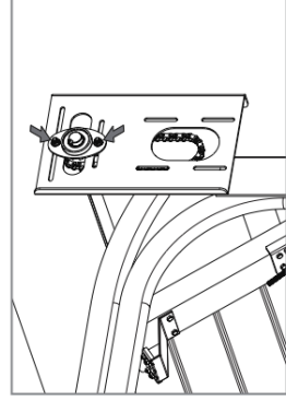
04 - Slightly loosen the bearing bracket's screws (left), to be able to move it sideways.
