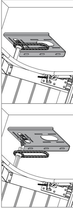
03 - Pass the \varnothing 25\text{mm} shaft through the bearing on the support plate.
