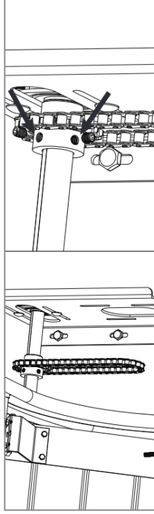
06 - Pull the pinion to the bearing and tighten the two bolts to secure the pinion to the shaft.
