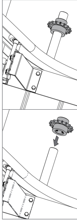
01 - Place the pinion on the \varnothing 25\text{mm} spring's shaft of the sectional door.
