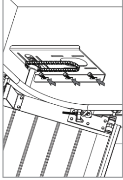
05 - Pull the metal plate to the wall and secure with the screws. After fixing the plate, tighten the bearing bracket's screws back to fix it too.
