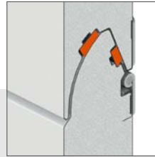
Panel with a thickness of 60 mm. U=0,9 \text{ [W/m}^2\text{K]}^*
